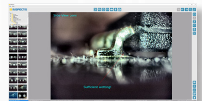
Wetting of the SOP pins
