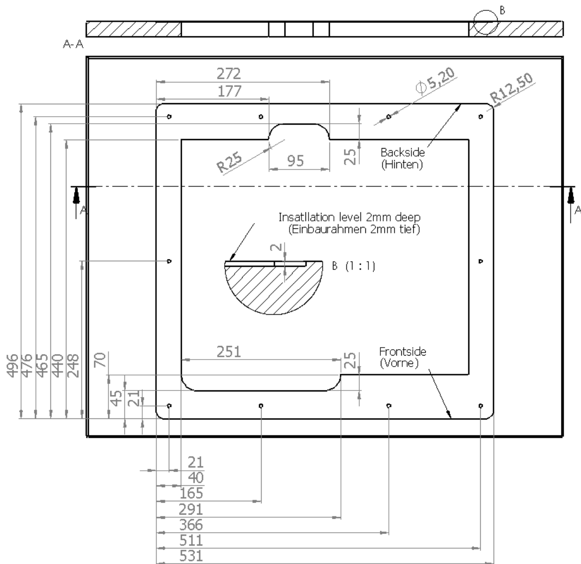
Fig. 61: Information for Work Surface Aperture HOTBEAM 05 Mounting Frame
