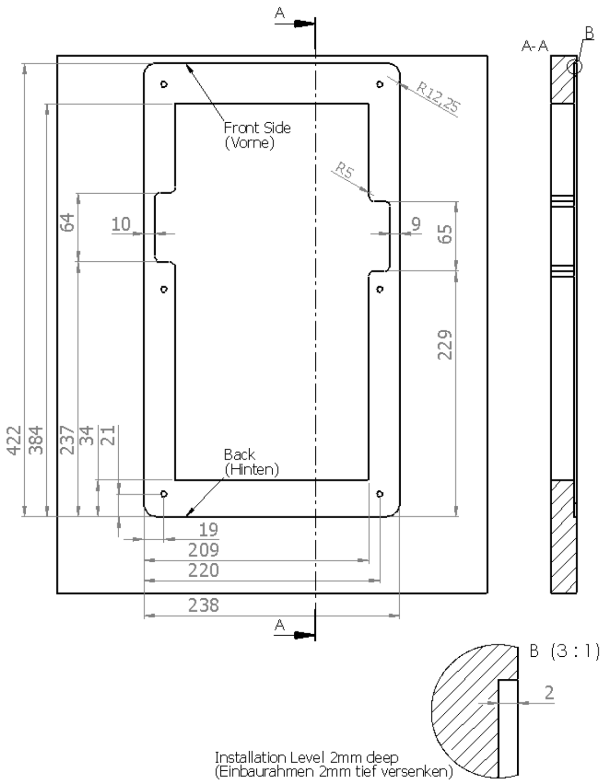
Fig. 59: Mounting Frame HOTBEAM 04
