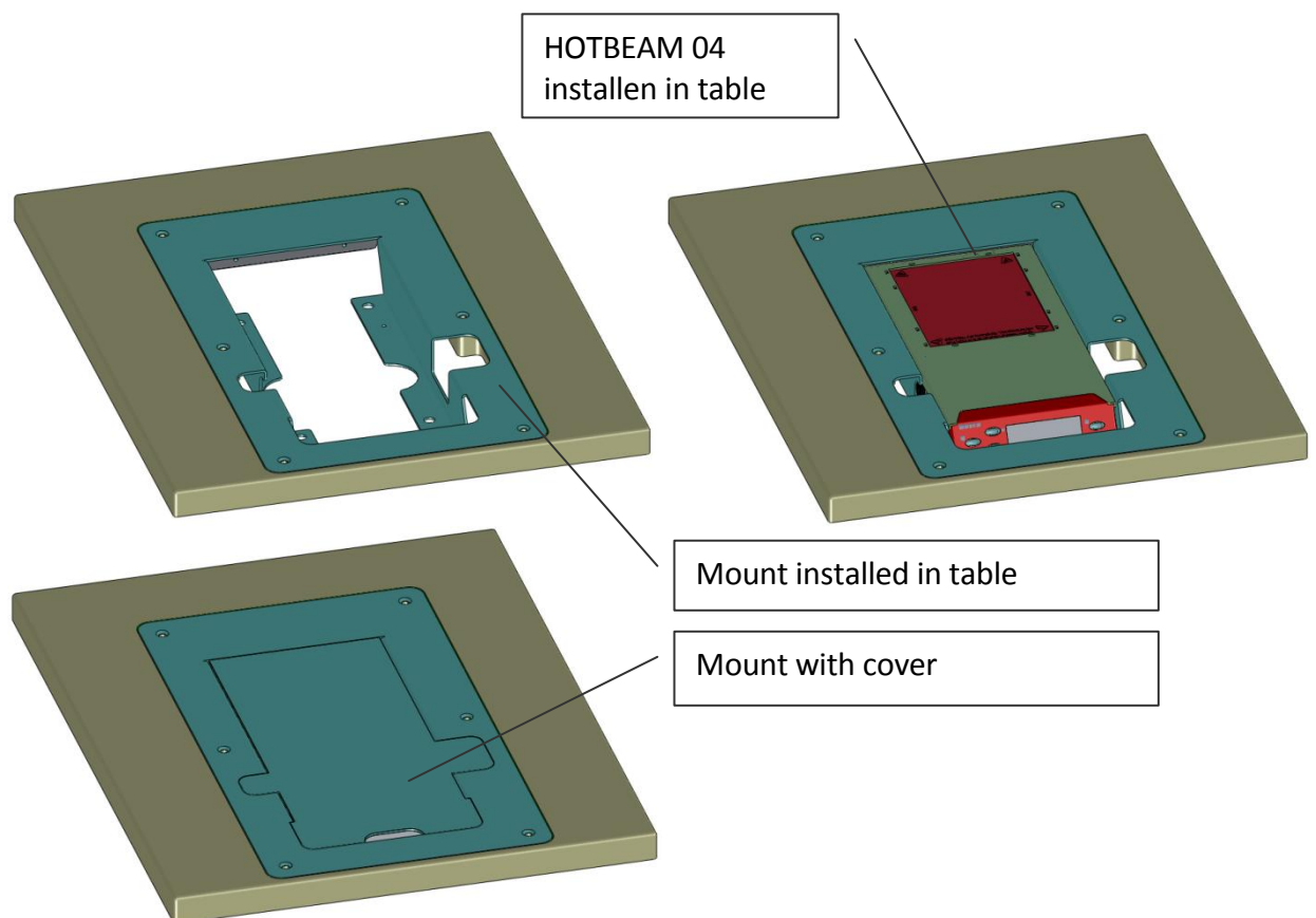
Fig. 58: Flush-mounting for HOTBEAM 04 with Mounting Frame
