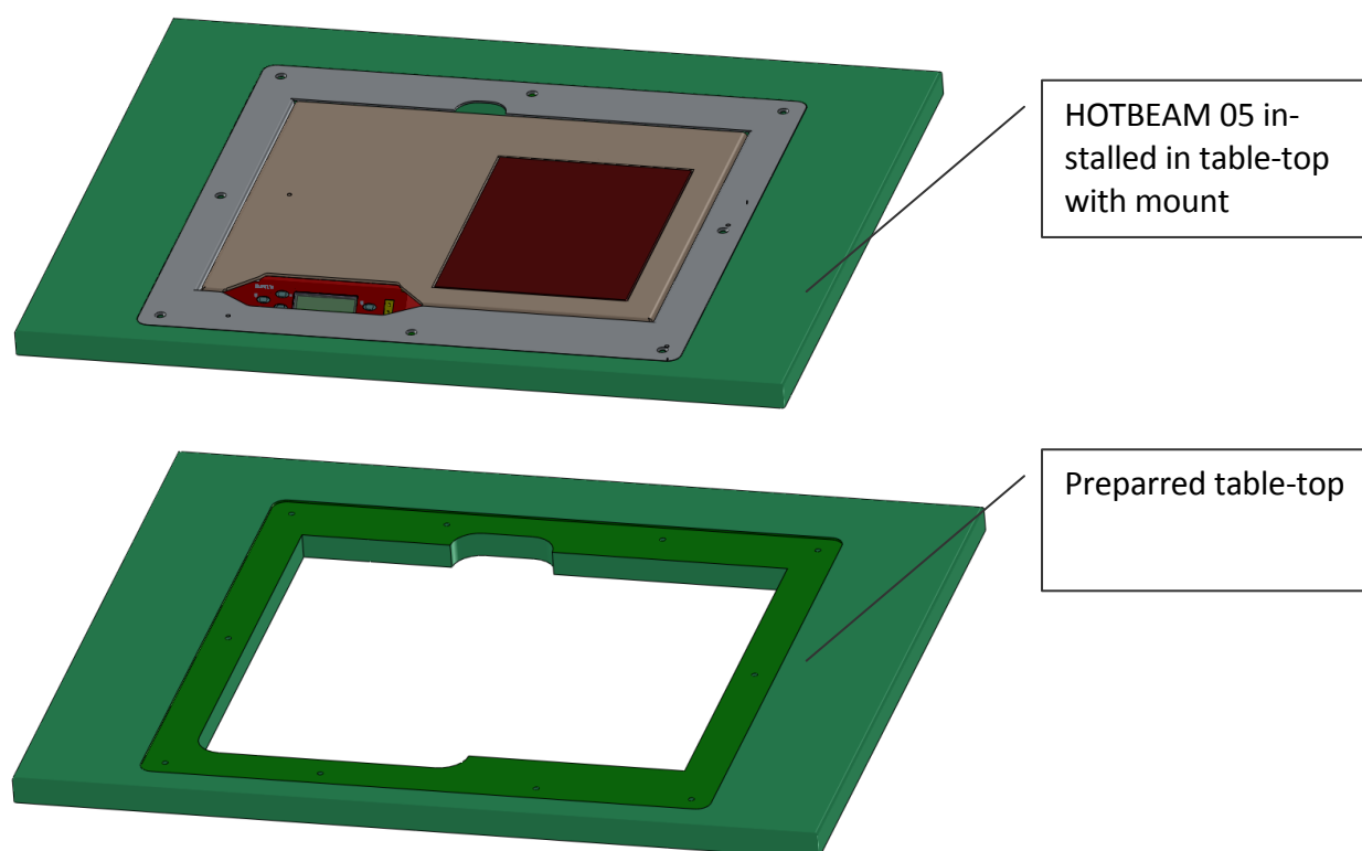
Fig. 60: Flush Mounting in Worktop HOTBEAM 05
